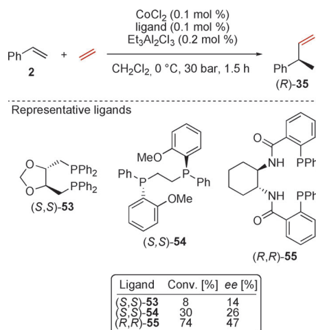
Scheme 17. Cobalt-catalyzed asymmetric styrene hydrovinylation reactions.
