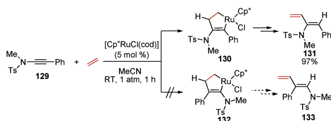
Scheme 29. A ruthenium-catalyzed intermolecular coupling reaction of ynamides and ethylene.
