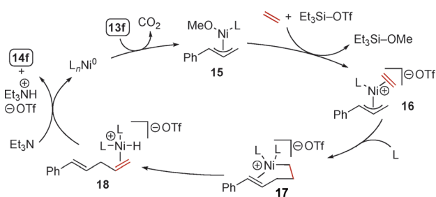
Scheme 5. Proposed mechanism of the nickel-catalyzed allylic substitution reactions using ethylene.
