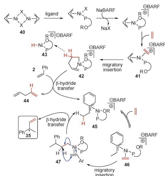
Scheme 14. The proposed mechanism of nickel-catalyzed hydrovinylation reactions of styrenes using hemilabile phosphine ligands.
