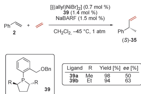
Scheme 13. Use of dialkylphospholanes in asymmetric hydrovinylation reactions of styrene.
