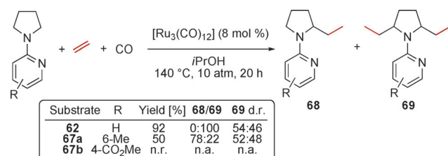
Scheme 20. Ruthenium-catalyzed \text{C}_{\text{sp}^3} -H ethylation reactions and their dependence on directing group functionality.
