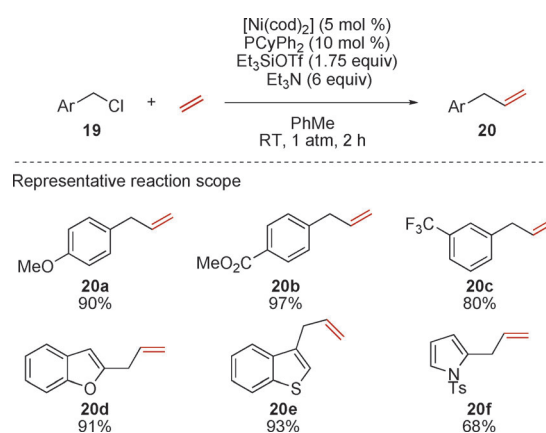
Scheme 6. Nickel-catalyzed benzylation and heterobenzylation reactions of ethylene.
