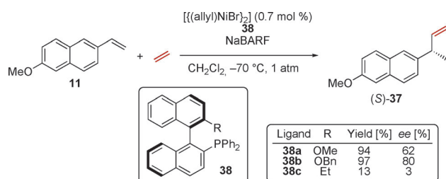
Scheme 12. The use of hemibidentate phosphine ligands in asymmetric hydrovinylation reactions.
