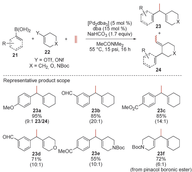
Scheme 7. Palladium-catalyzed three-component couplings of ethylene to boronic acids and vinyl triflates and vinyl nonaflates. Boc = tert -butoxycarbonyl.
