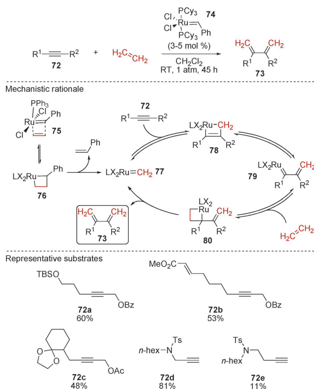
Scheme 22. Ruthenium-catalyzed enyne metathesis reactions using ethylene as the alkene substrate. Bz = benzoyl, TBS = tert-butyldimethylsilyl.
