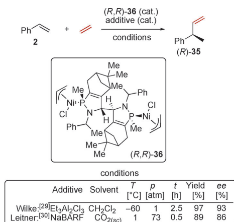
Scheme 11. The use of pinene-derived azaphospholene ligands in asymmetric hydrovinylation reactions of styrene.
