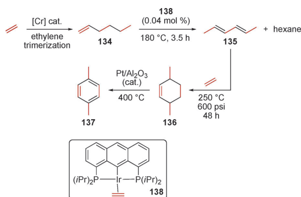
Scheme 30. Brookhart's ethylene-based p -xylene synthesis.
