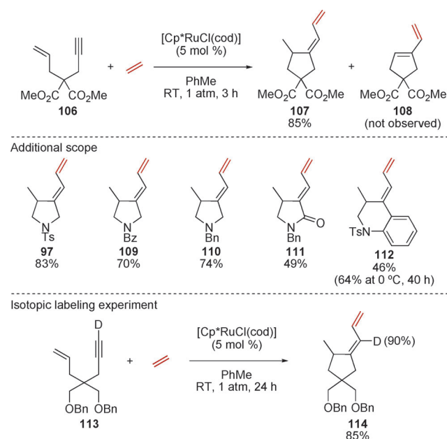
Scheme 27. Optimization, scope, and mechanistic study of the ruthenium-catalyzed oxidative cyclization/exocyclic diene formation from diterminal 1,6-enynes.
