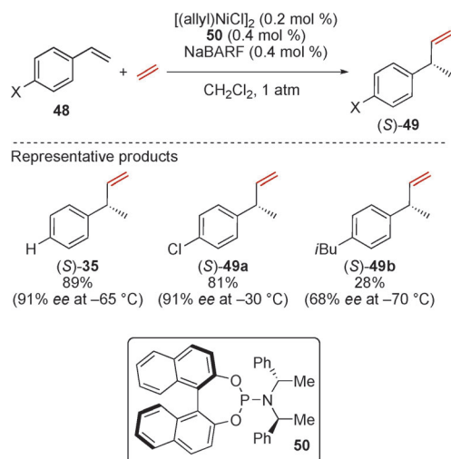
Scheme 15. The use of phosphoramidite ligands in the asymmetric hydrovinylation of styrenes.
