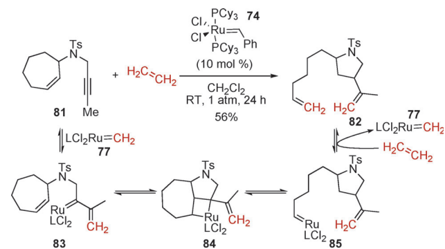
Scheme 23. Ruthenium-catalyzed ring-closing/ring-opening reactions of alkynes with tethered cyclic alkenes in the presence of ethylene.
