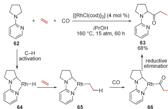
Scheme 19. The rhodium-catalyzed three-component \text{C}_{\text{sp}^3}\text{–H} functionalization of N -(2-pyridyl)pyrrolidine using ethylene and carbon monoxide.
