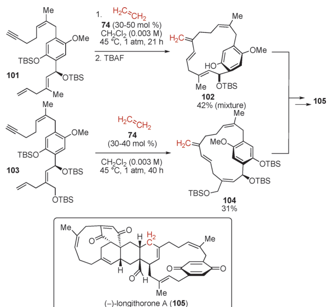
Scheme 26. Application of ethylene-incorporating ring-closing enyne metathesis reactivity to the total synthesis of (–)-longithorone A. TBAF = tetra- n -butylammonium fluoride.
