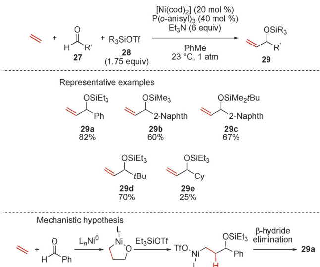
Scheme 9. Nickel-catalyzed three-component couplings of ethylene to aldehydes and silyl triflates.
