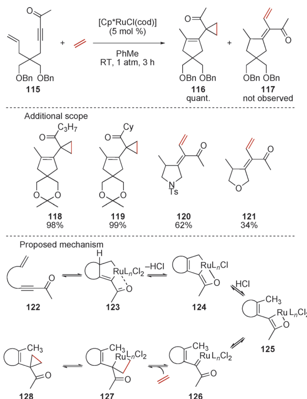
Scheme 28. The scope and proposed mechanism of the ruthenium(II)-catalyzed tandem cyclopentene/cyclopropanation reaction of internal alkyne-containing 1,6-enynes.
