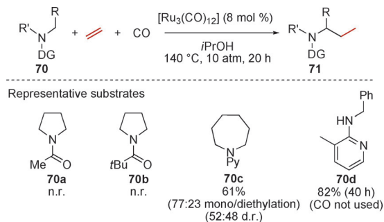
Scheme 21. Additional substrate scope of directed ruthenium-catalyzed C–H ethylation reactions. DG = directing group, Py = pyridyl.
