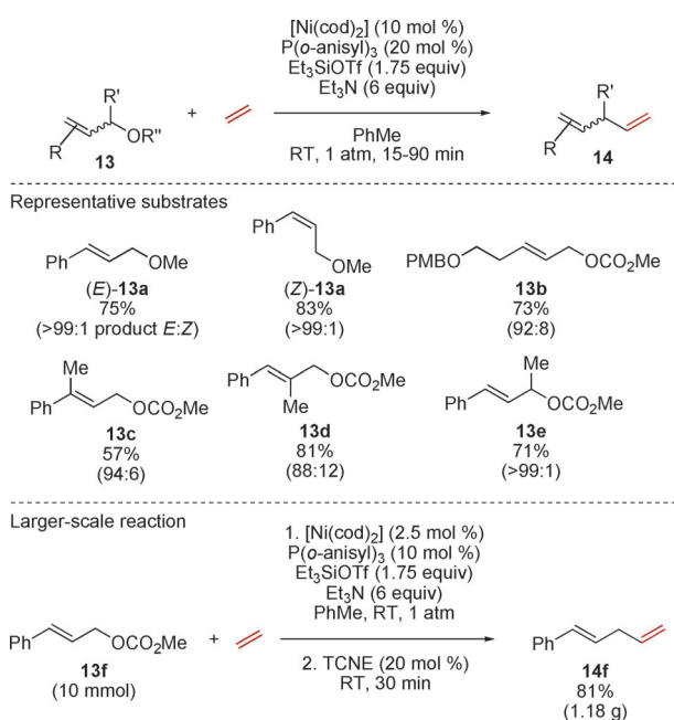
Scheme 4. Nickel-catalyzed substitution reactions of allylic electrophiles with ethylene. cod = 1,5-cyclooctadiene, PMB = para -methoxybenzyl, TCNE = tetracyanoethylene, Tf = trifluoromethanesulfonyl.
