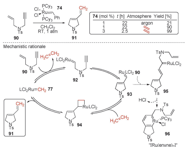
Scheme 24. An ethylene-mediated ruthenium-catalyzed intramolecular enyne metathesis reaction.
