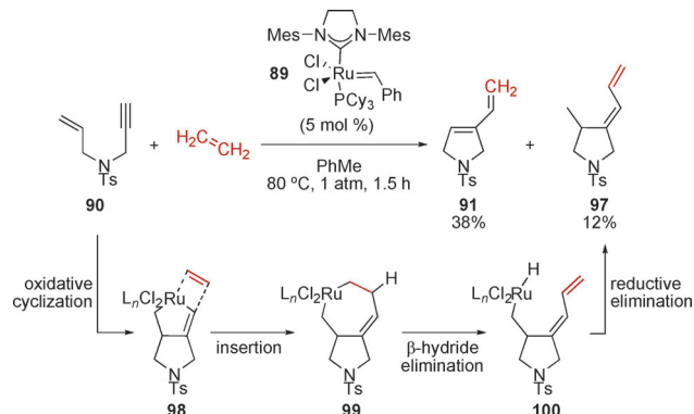
Scheme 25. Oxidative cyclization of an enyne metathesis substrate in the presence of ethylene and Grubbs's second-generation catalyst.
