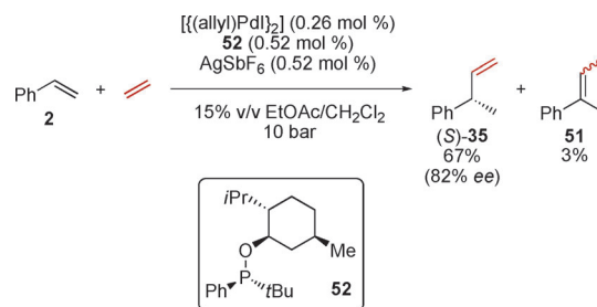
Scheme 16. The use of menthol-derived phosphonite ligands in palladium-catalyzed asymmetric hydrovinylation reactions.
