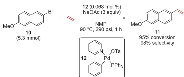
Scheme 3. The C,N-palladacycle-catalyzed Mizoroki–Heck arylation of 2-bromo-6-methoxynaphthalene. NMP = 1-methyl-2-pyrrolidone, Ts = 4-toluenesulfonyl.
