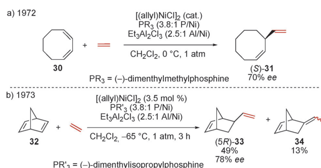
Scheme 10. Wilke's protocol for the asymmetric hydrovinylation of biased alkenes.
