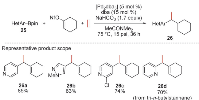
Scheme 8. The use of heteroaromatic transmetalating reagents in palladium-catalyzed three-component couplings of ethylene to boronic acids and vinyl nonaflates. pin = pinacol.
