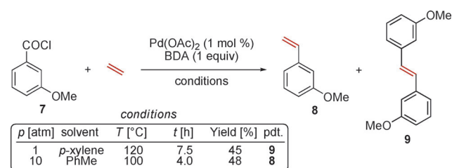
Scheme 2. Palladium-catalyzed Mizoroki–Heck arylations of ethylene using benzoyl chloride electrophiles. BDA = benzyldimethylamine.
