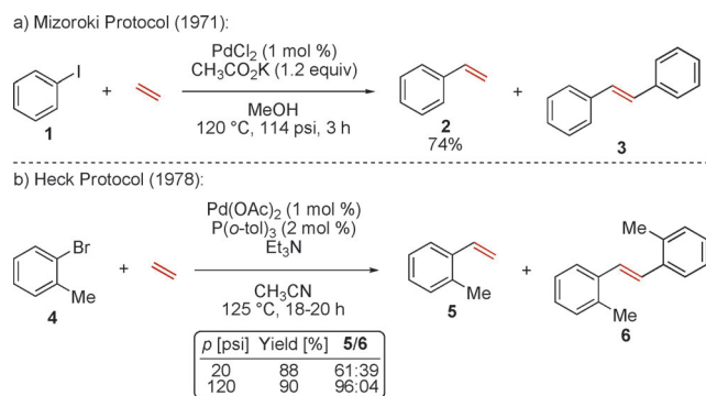
Scheme 1. Palladium-catalyzed Mizoroki–Heck arylations of ethylene.
