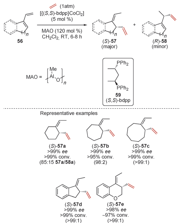
Scheme 18. Cobalt-catalyzed 1,4-hydrovinylation reactions of vinylcycloalkenes.
